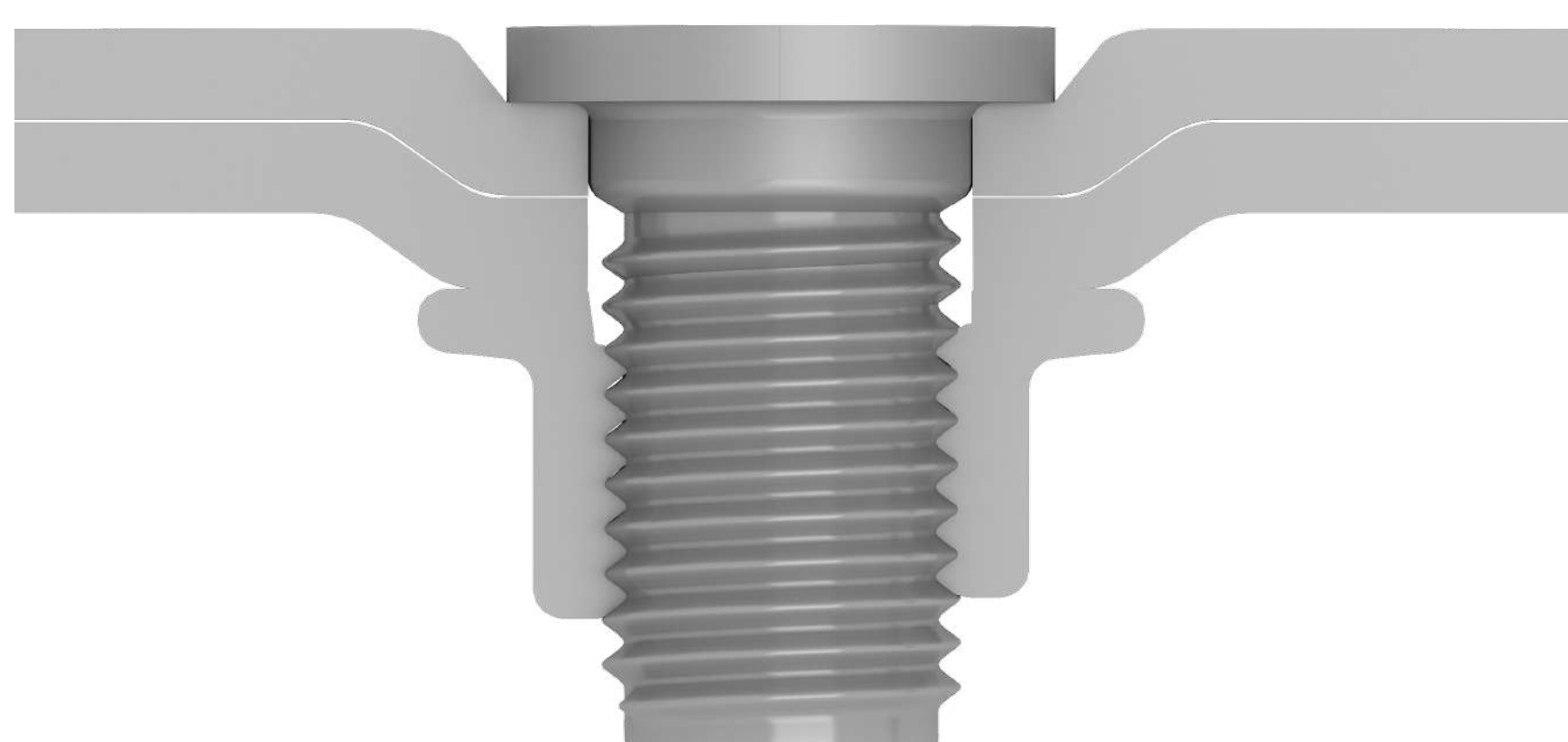
Sigmat 'Flush Finish'
